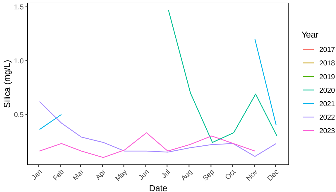
B2 Raceway 1 Silica (mg/L) Monthly Statistics
